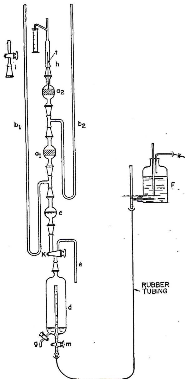
Apparatus for the Determination of the Liquid Permeability of Glass Filters and Core Samples.
