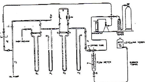
Permeability Apparatus for Low Pressures.
