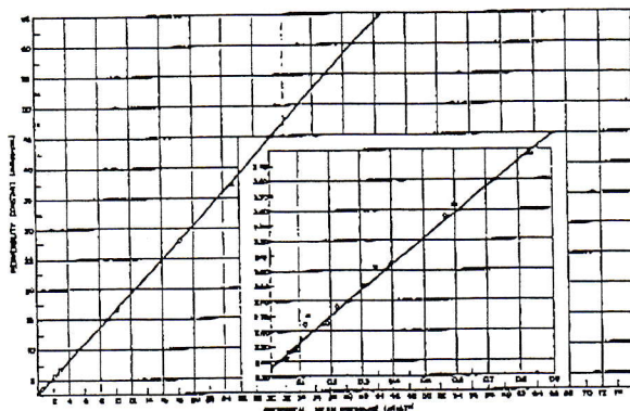
Permeability Constant of Jens Glass Filter G4A to Air at Different Pressures (Permeability Constant to Isooctane, 2.36 Md).
