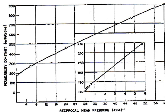
Permeability Constant of Core Sample "F" to Air at Different Pressures (Permeability Constant to Isooctane, 170 Md).
