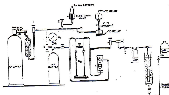
Permeability Apparatus for High Pressures.
